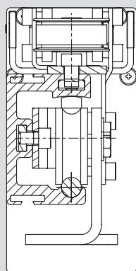
Cross section
