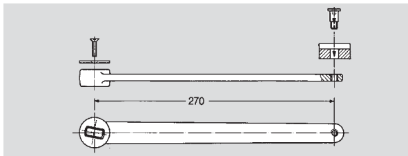
Swing lever Art. No. 7451 N
