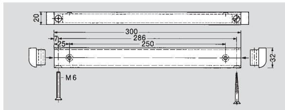
Guide housing Art. No. 7453 N
