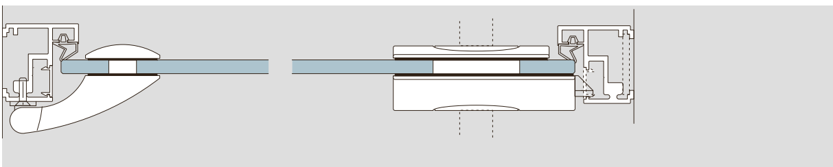
ALEXA AT 44 - mit ARCOS Office ALEXA AT 44 - with ARCOS Office
