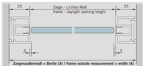
Grundriss / Tür / plan / door
