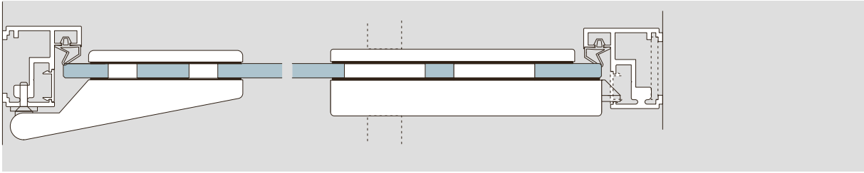
ALEXA AT 44 - mit DORMA Studio (Classic, Rondo) ALEXA AT 44 - with DORMA Studio (Classic, Rondo)
