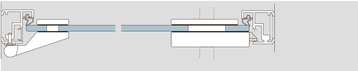
ALEXA AT 44 - mit DORMA Junior (Office, Office Classic) ALEXA AT 44 - with DORMA Junior (Office, Office Classic)
