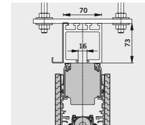
K-type track Mechanically coded junction technology with curves and switches for easy operation; suitable for element weights up to 250 kg.
