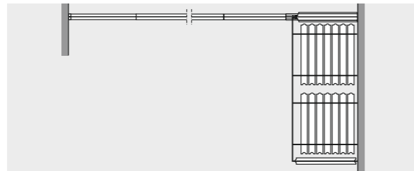
Parking solution PLC – Two-point suspension – 90° to partition axis – In several stacks – Here with telescopic wall abutment AWA and two-sided stack closure element
