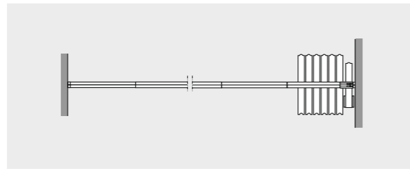
Parking solution PLA – Single-point suspension – 90° to partition axis
