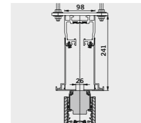
ComfortDrive Fully automatic track operator system. Fast opening and closing speeds of up to 250mm/s for enhanced convenience. Easy pushbutton operation. Narrow profiles for aesthetic elegance. The
