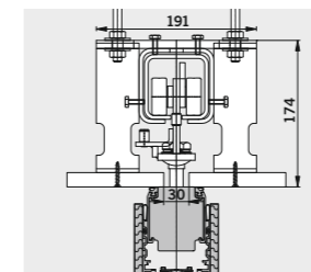
SmartTrack Steel track system for large element heights and high weights, with special mechanical coding in the carriers, plus curves and switches for maximum operating ease and effortless positioning of
