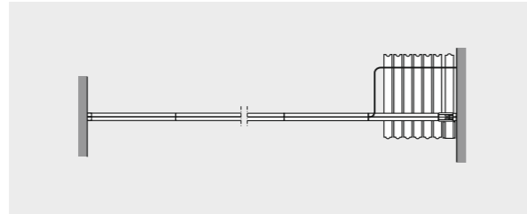
Parking solution PLB – Two-point suspension – 90° to partition axis
