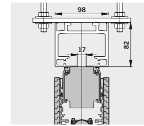
R-type track Track system for right-angled configurations with cross-roller carriers for element weights up to 500 kg. Support rollers in the junctions guarantee easy operation
